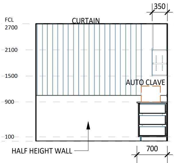
3 ELEVATION DETAIL 1 : 50
