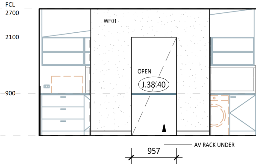
5 ELEVATION DETAIL 1 : 50
