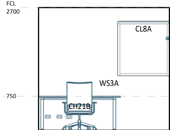
8 ELEVATION DETAIL 1 : 50
