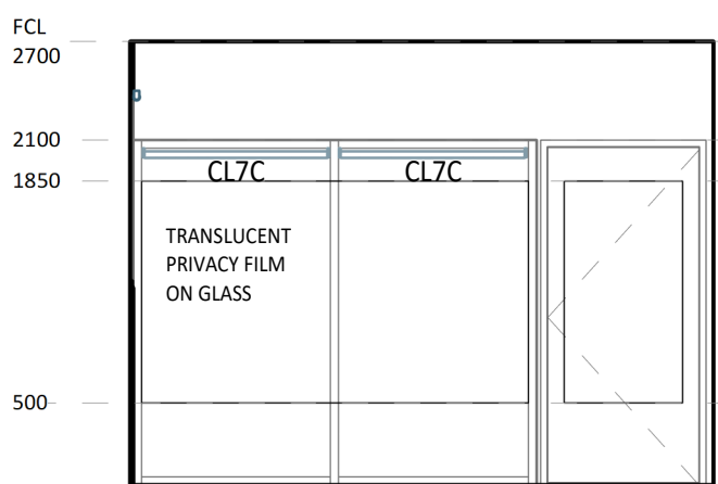
7 ELEVATION DETAIL 1 : 50
