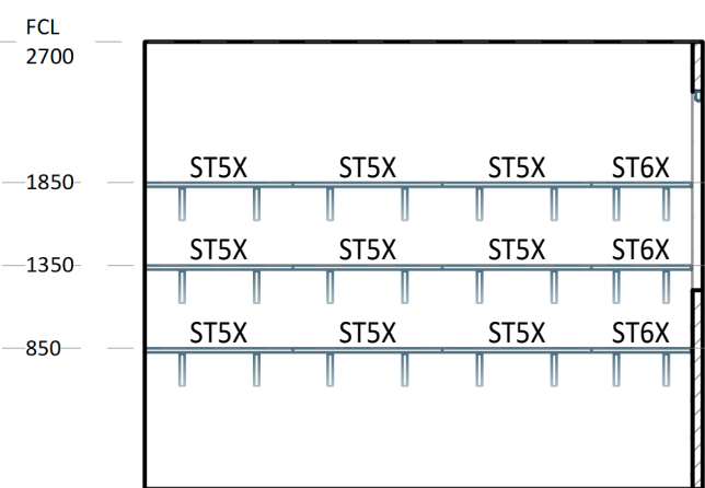
9 ELEVATION DETAIL 1 : 50
